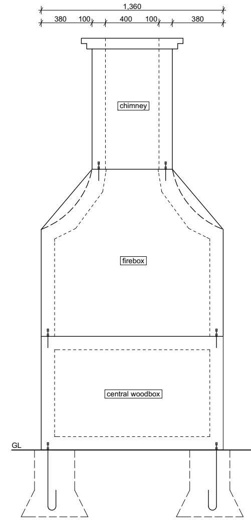
Rear Elevation
