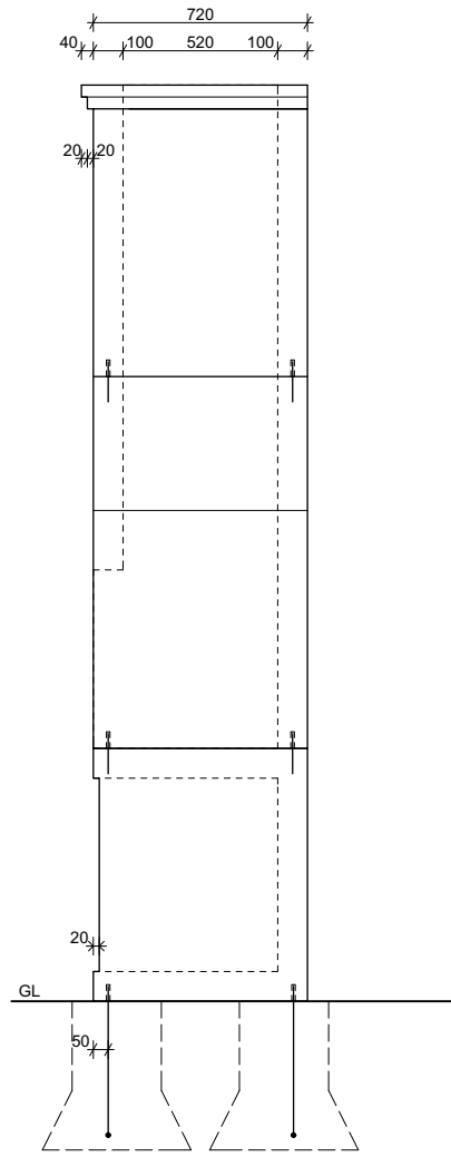
Side Elevation
